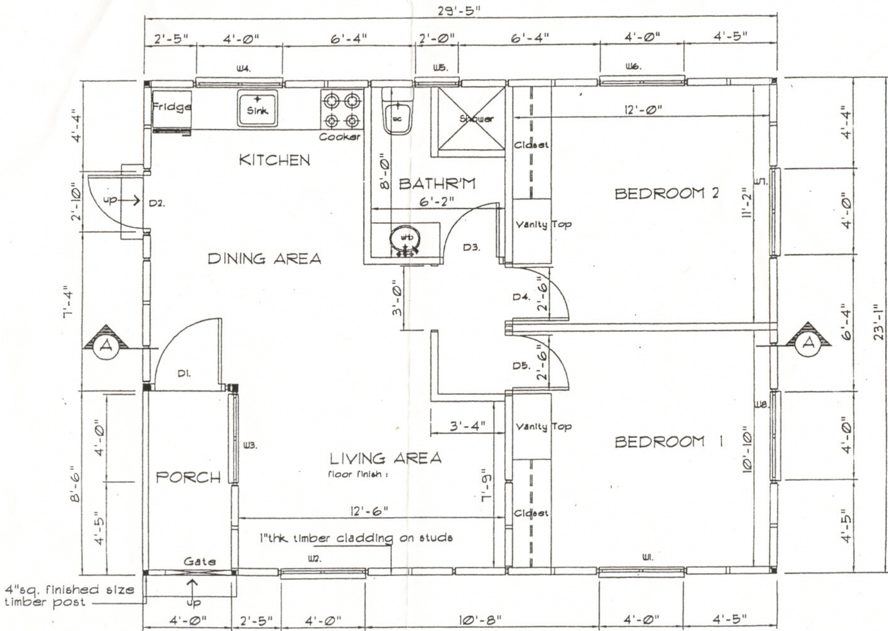
REVISED TWO BEDROOM UNIT Area = (679.60 sq.ft.)
